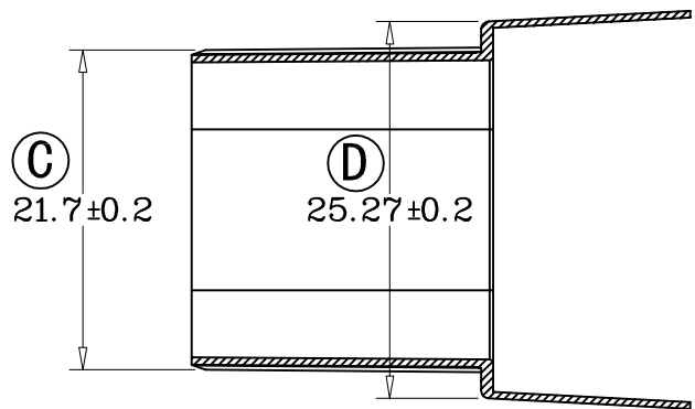
VIEW: A-A
